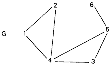
Figure 1. — G is an interval graph since there exists a numbering of its nodes such that the adjacency matrix A verifies the property (\mathcal{P}) .
