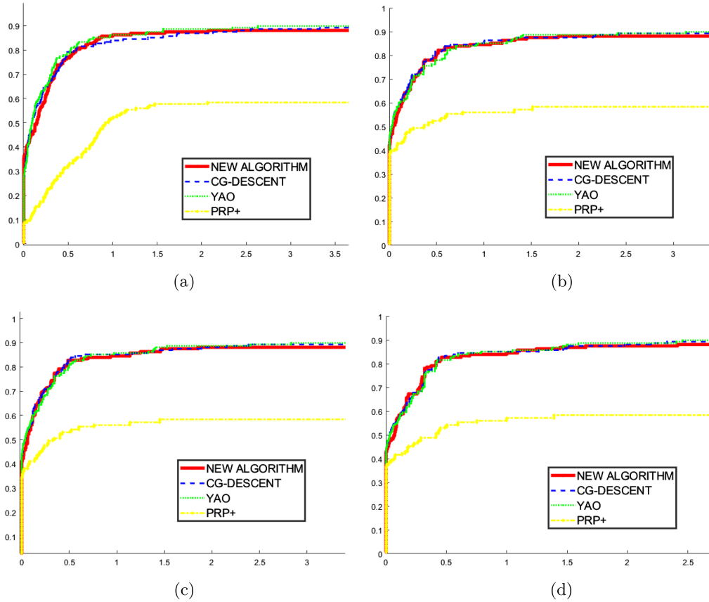
FIGURE 1. The performance profile on the CPU time (a), the number of iterations (b), the number of function evaluations (c) and the number of gradient evaluations (d).
