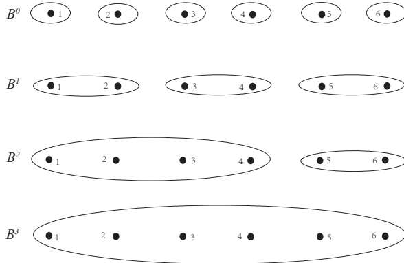
Fig. 1 \mathcal{B} in Example 1
