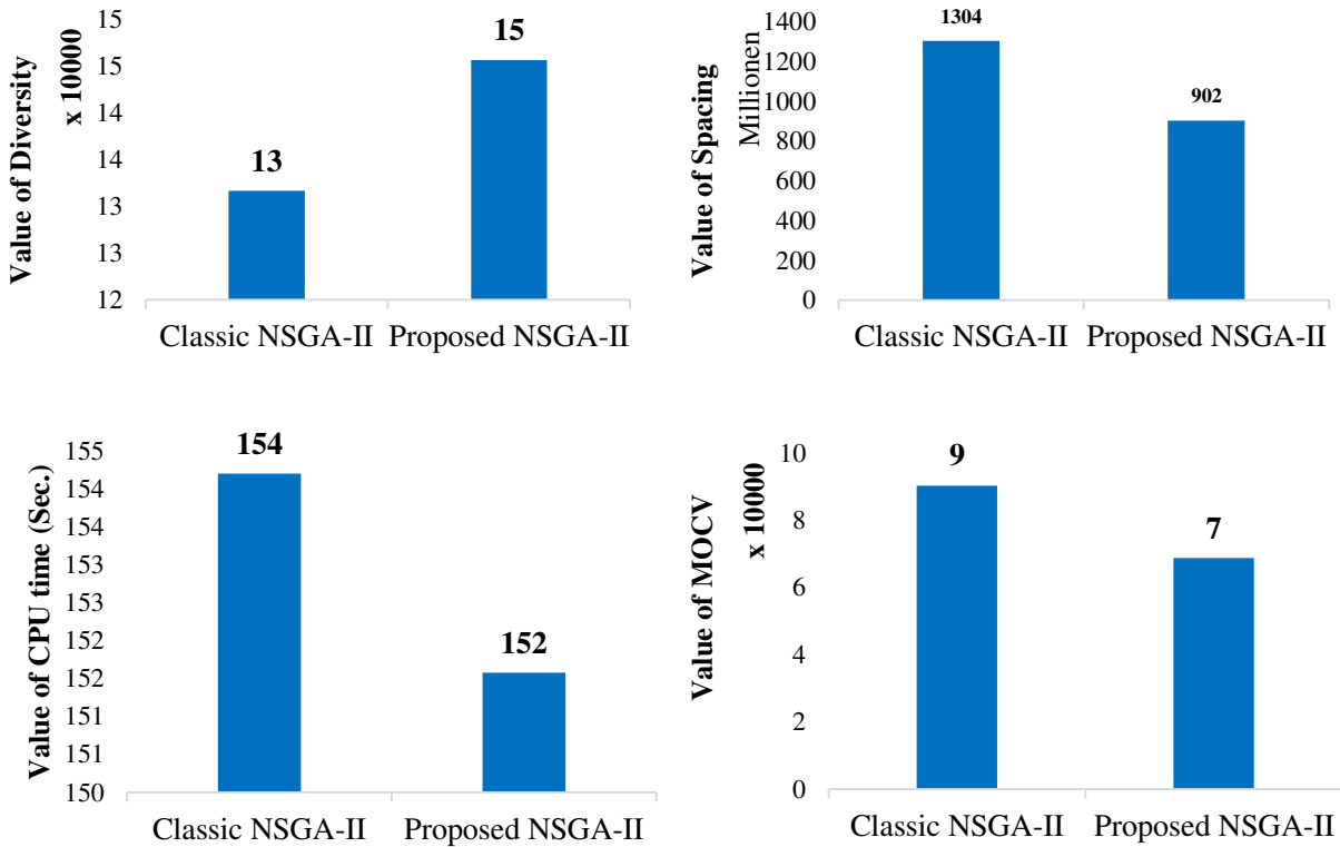
Figure 16: Performance metrics comparison in classic NSGA-II and proposed NSGA-II
