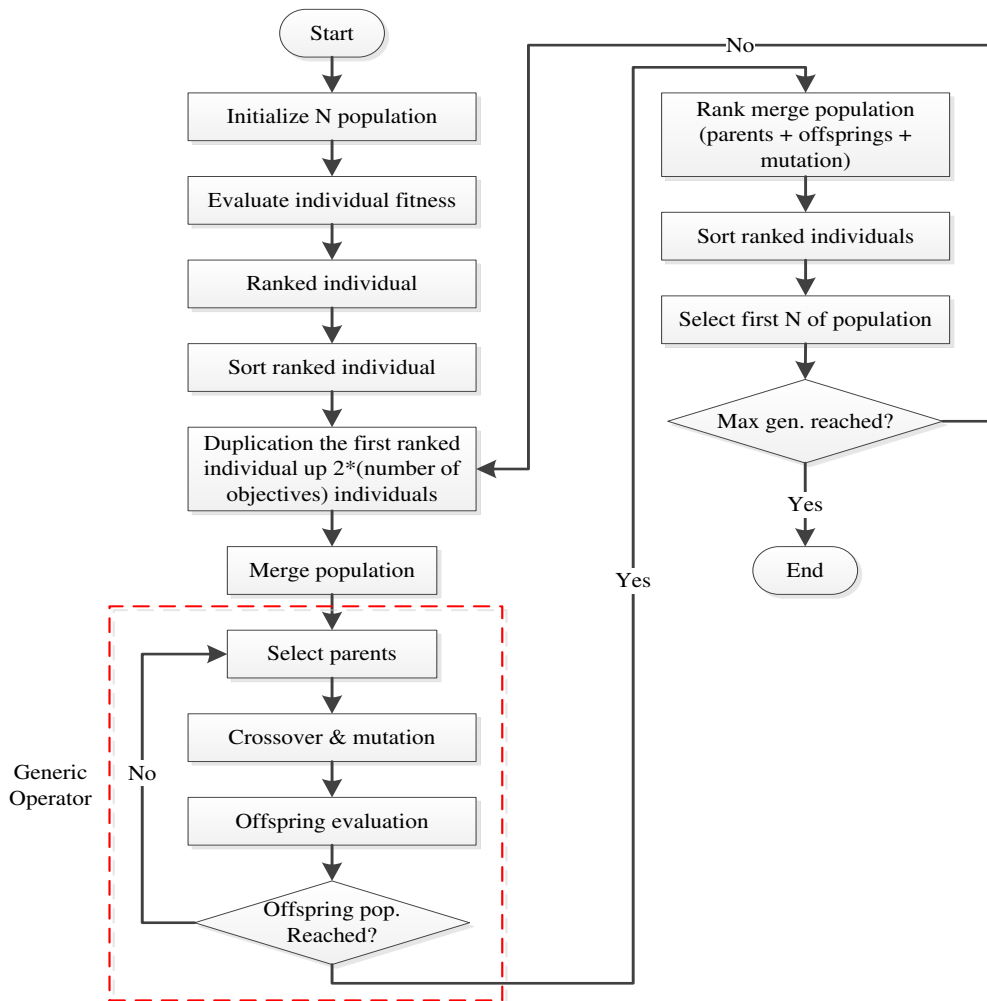
Figure 2: Proposed NSGA-II algorithm
