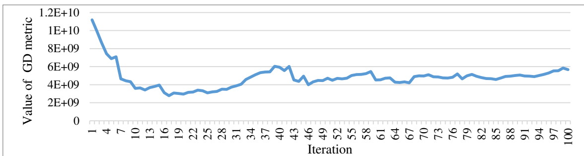
Figure 19: Variety of GD metric value during iterations
