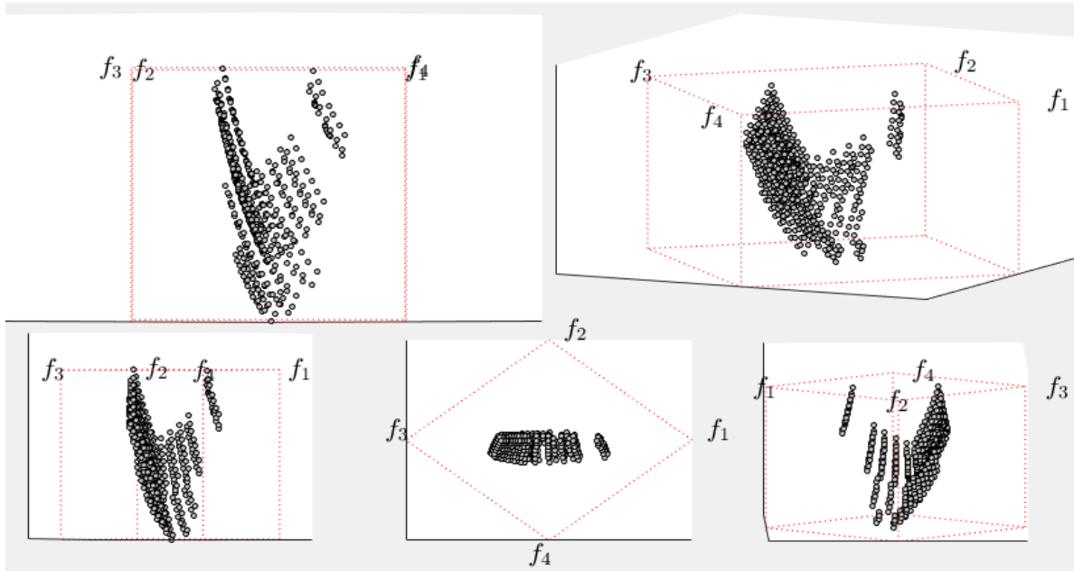
Figure 11: Pareto-optimal space in 3D-RadVis figure
