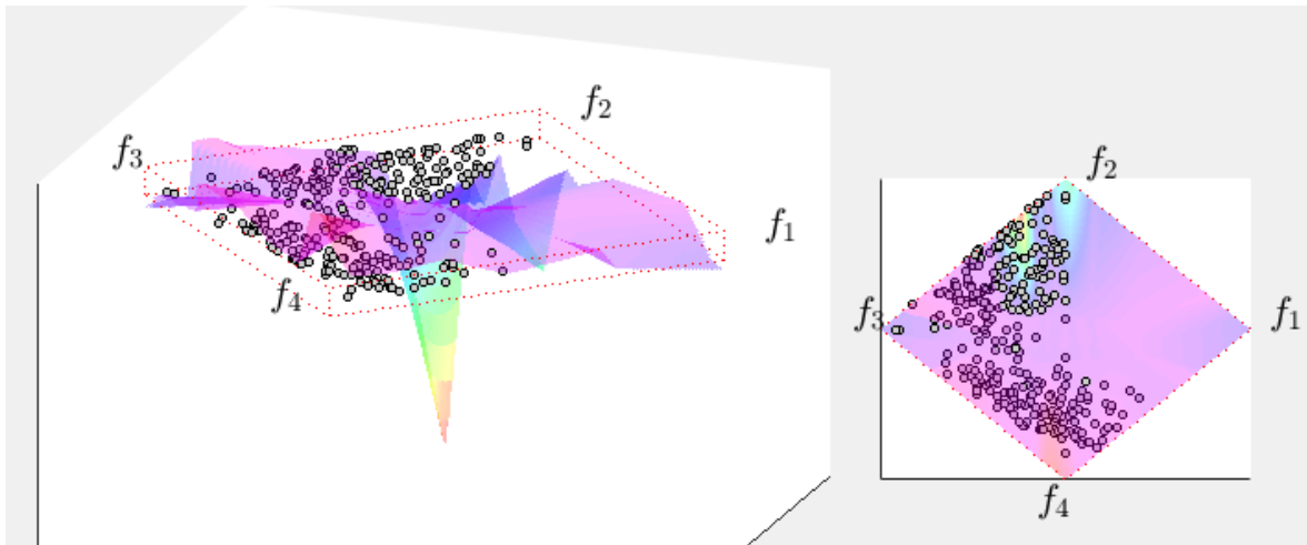
Figure 17: Graphical demonstration of true Pareto front and NSGA-II solutions in 3D-RadVis
