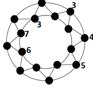
Figure 3: The illustration of T(C_8) when (a_1, a_2) = (4, 1) and T(C_8)[V_4 \cup \dots \cup V_7] \cong 2K_2 .
