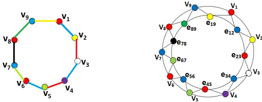
Figure 4: A min-TDTC of C_9 (left) and the corresponding min-TDTC of T(C_9) (right).
