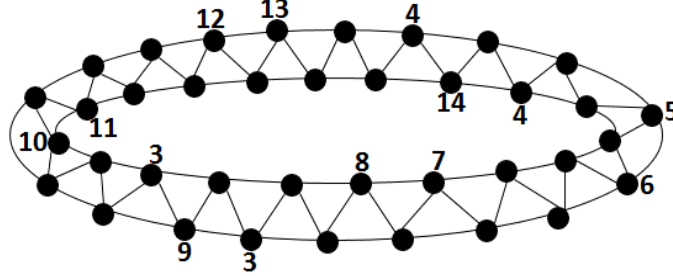
Figure 6: The illustration of T(C_{19}) when (a_1, a_2) = (10, 2) , T(C_{19})[V_5 \cup \dots \cup V_{14}] \cong \overline{K_2} \cup \mathcal{H}_8 and |\bigcup_{i=3}^{14} CN(V_i)| = 38 .
